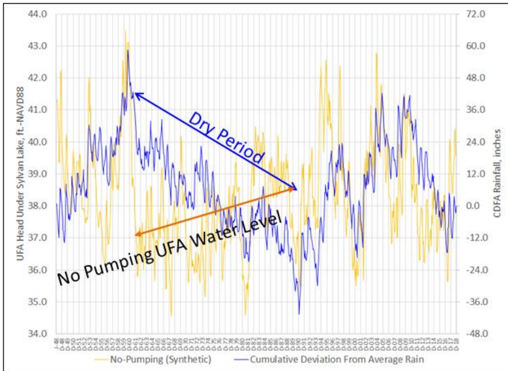
Figure 1. Sylvan Lake NP UFA Head Series and Rainfall.
