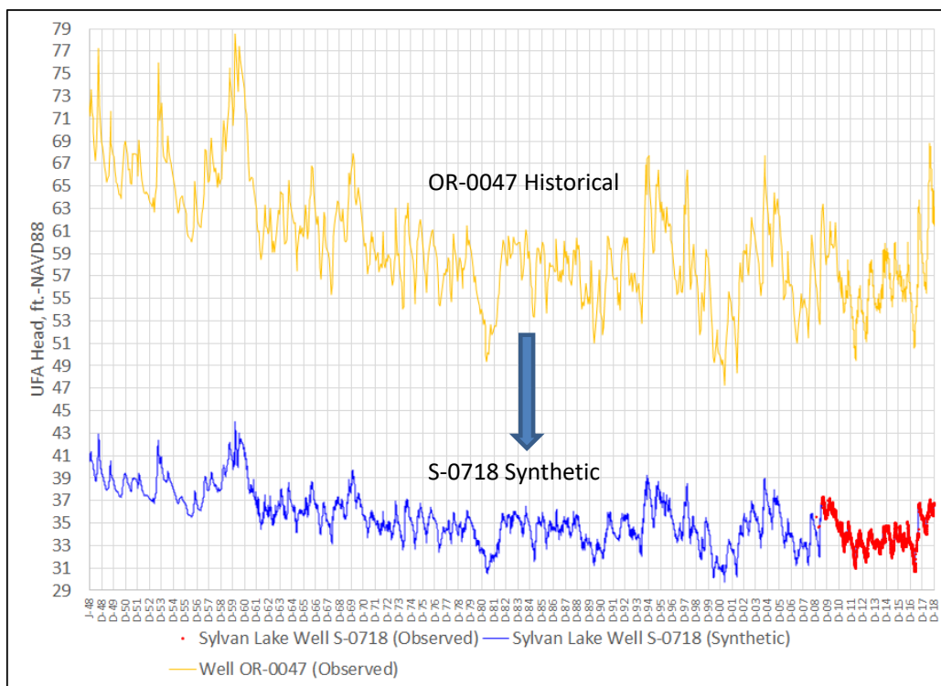
Figure 2. Extension of UFA head series near Sylvan Lake (Well S-0718).
