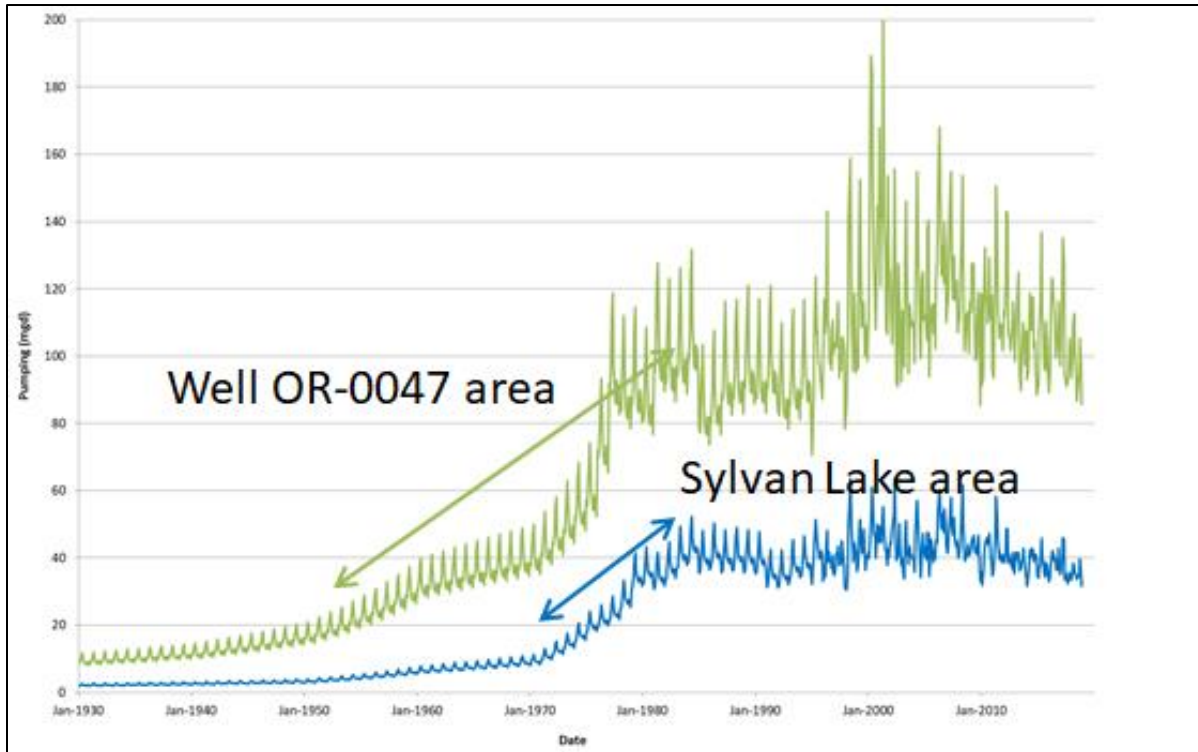
Figure 4. Historical Pumpage near Well OR-0047 and Well S-0718.
