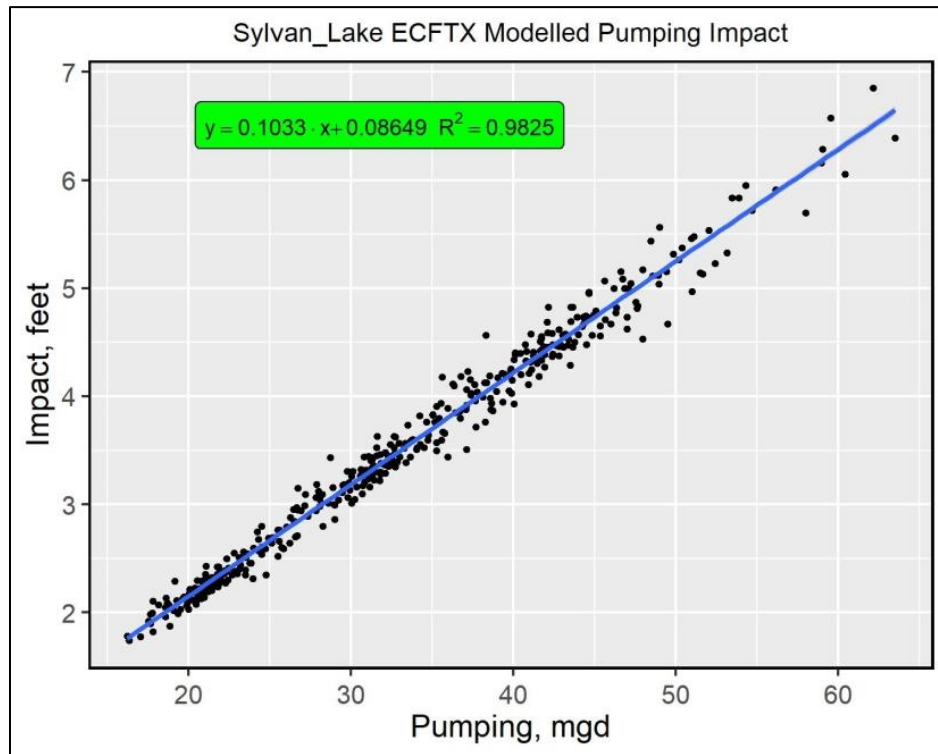
Figure 5. Linear Regression Used to Estimate UFA Historical Impacts for Conversion from Historical Conditions to NP Conditions.
