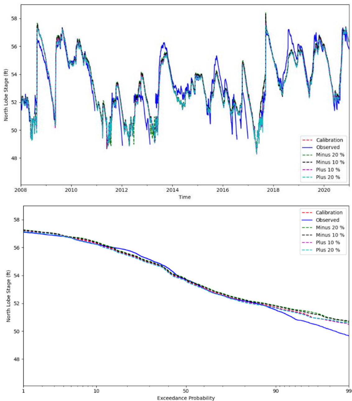
Figure 27. Impact of LZSN on simulated stages of the North Lobe of Prevatt Lake
