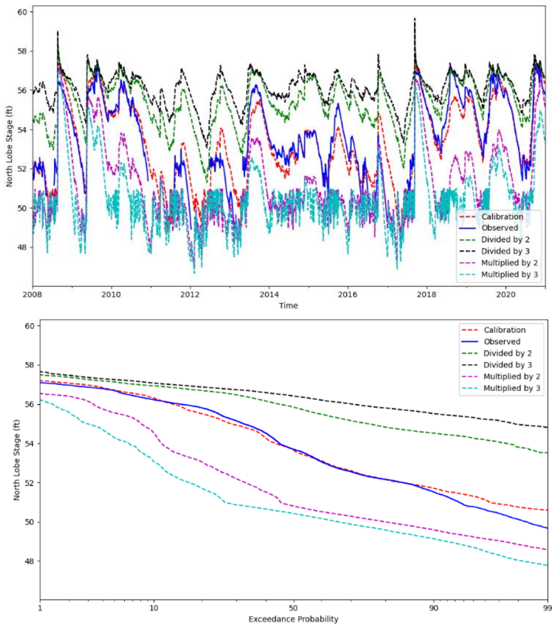
Figure 25. Impact of leakance value on simulated stages of the North Lobe of Prevatt Lake
