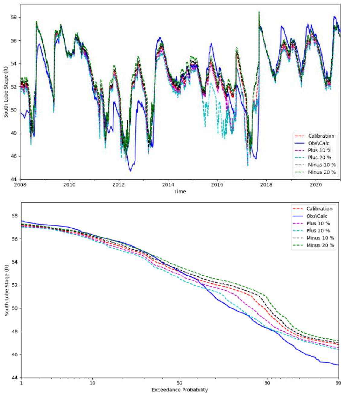
Figure 32. Impact of LZETP on simulated stages of the South Lobe of Prevatt Lake
