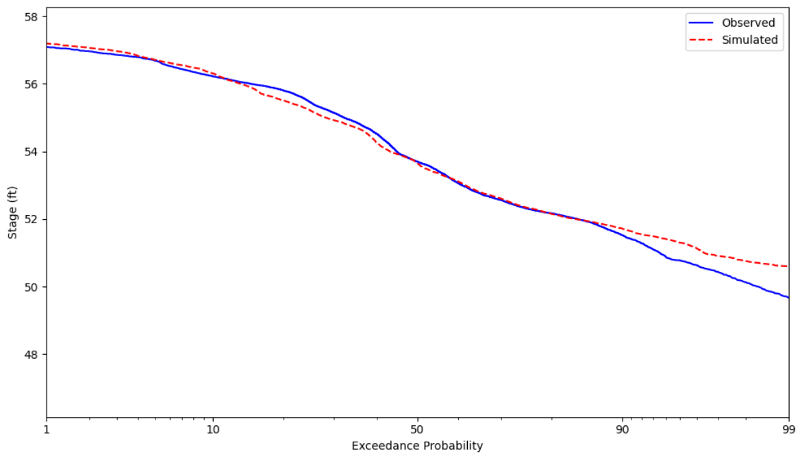
Figure 18. Observed and simulated daily stage duration curves for North Lobe for calibration period
