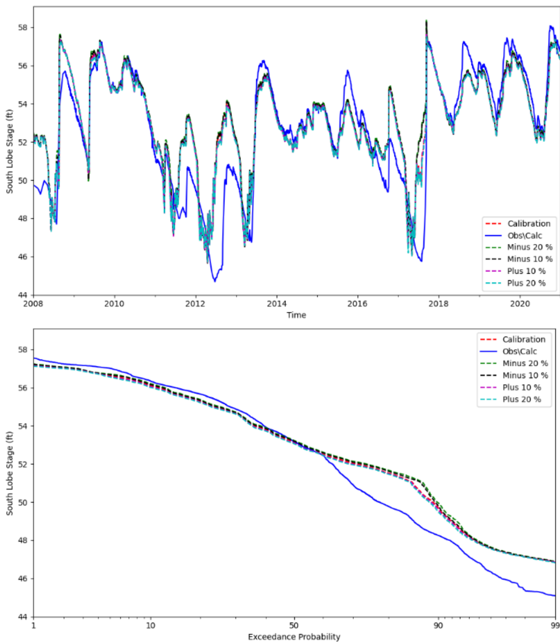
Figure 28. Impact of LZSN on simulated stages of the South Lobe of Prevatt Lake
