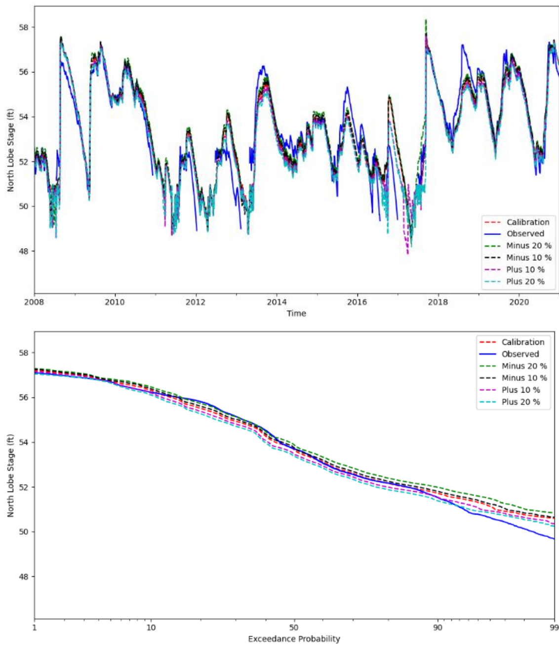
Figure 29. Impact of DEEPFR on simulated stages of the North Lobe of Prevatt Lake
