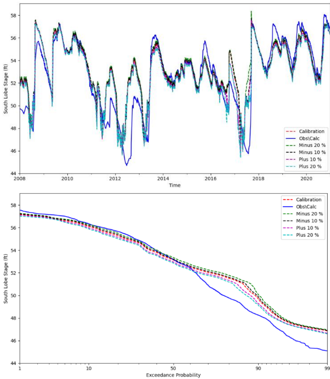
Figure 30. Impact of DEEPFR on simulated stages of the South Lobe of Prevatt Lake
