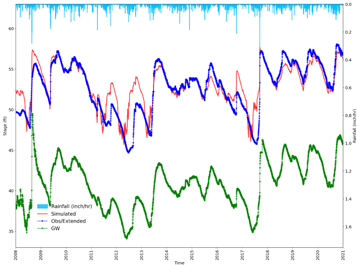
Figure 19. Observed/extended and simulated daily stages for the South Lobe of Prevatt Lake for calibration period
