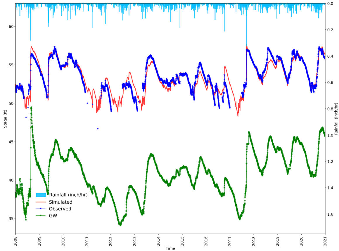
Figure 17. Observed and simulated daily stages for the North Lobe of Prevatt Lake for calibration period
