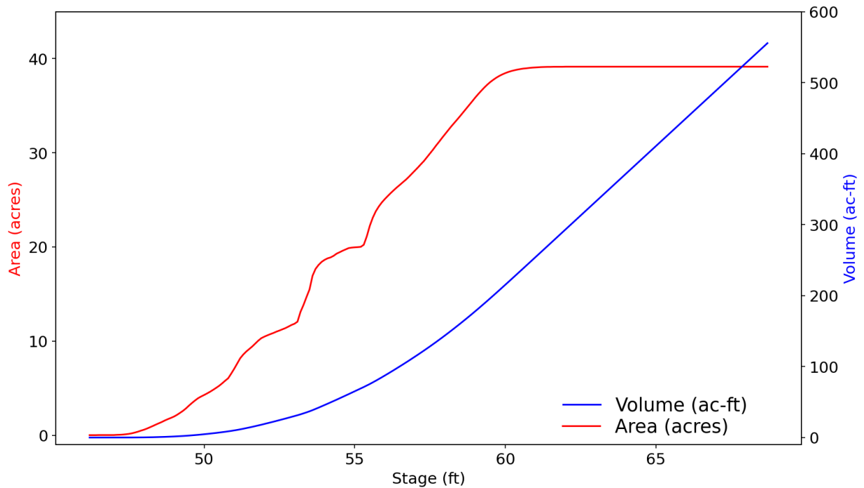
Figure 15. Stage-Area and Stage-Volume relationship for the North Lobe
