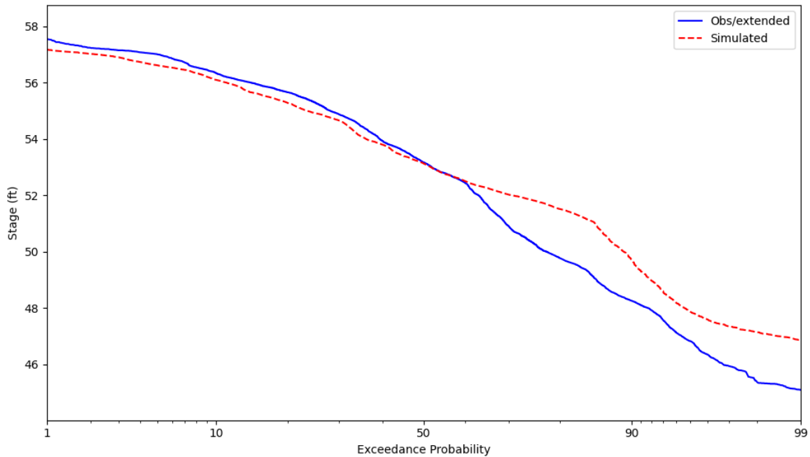
Figure 20. Observed and simulated daily stage duration curves for South Lobe for calibration period
