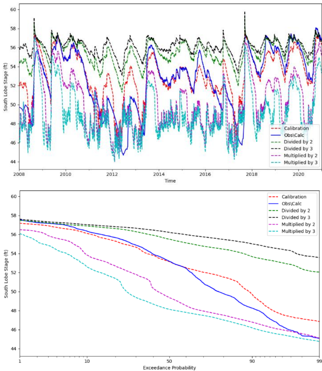
Figure 26. Impact of leakance value on simulated stages of the South Lobe of Prevatt Lake
