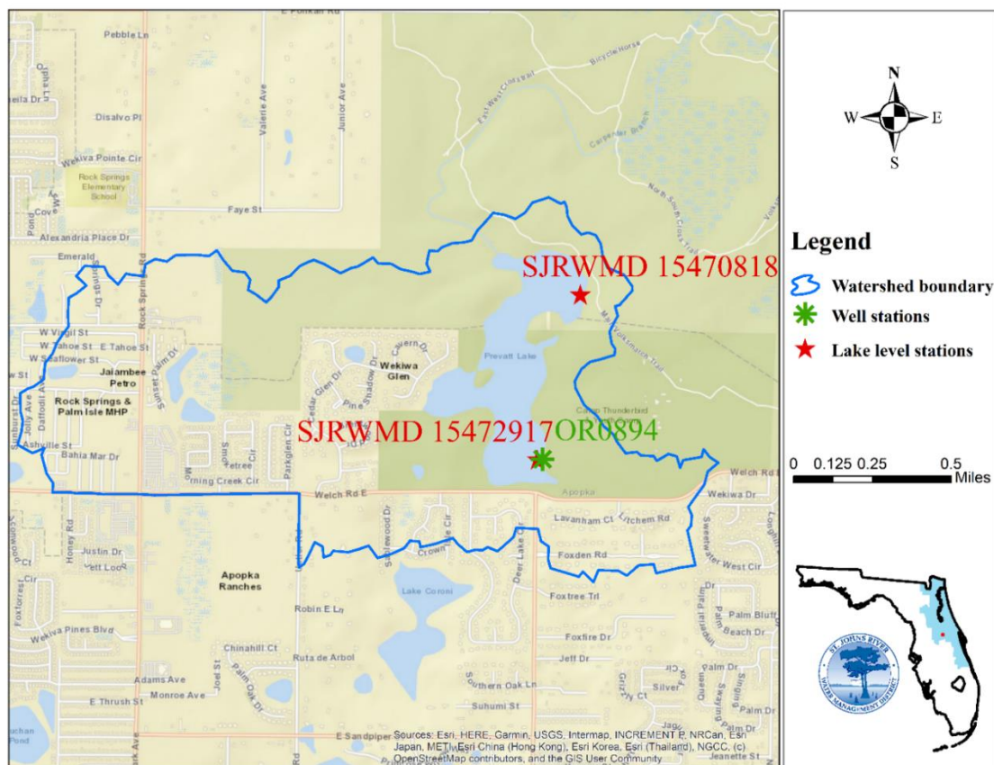
Figure 7. Stage recorders and surficial aquifer well locations
