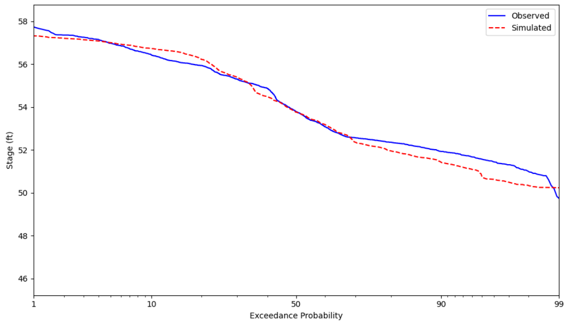
Figure 22. Observed and simulated daily stage duration curves for North Lobe for validation period
