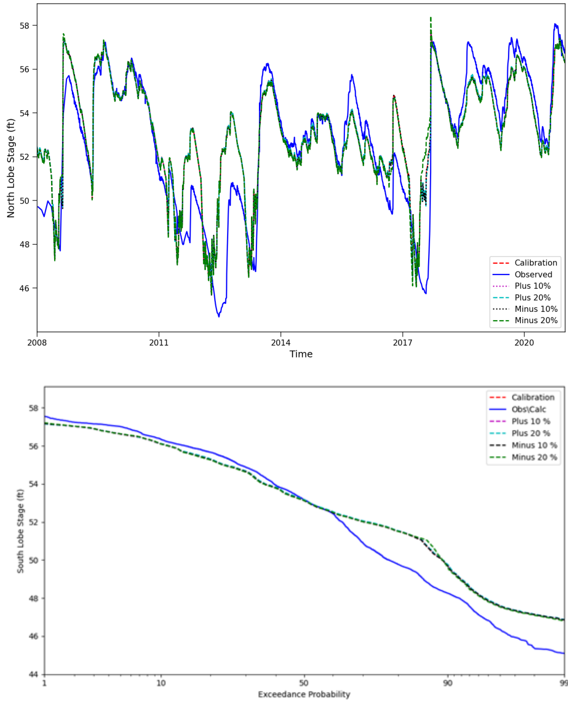
Figure 34. Impact of INFILT on simulated stages of the South Lobe of Prevatt Lake
