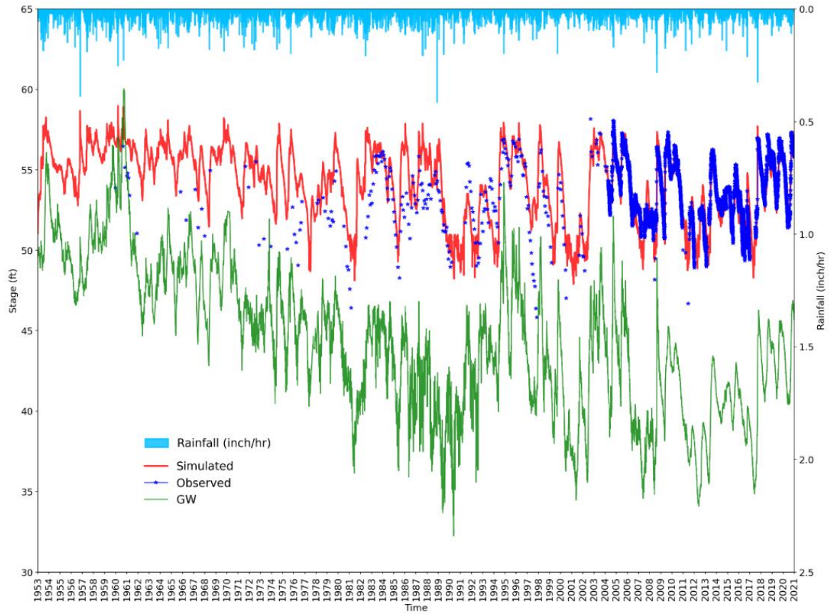
Figure 23. Daily long-term observed and simulated stages of the North Lobe of Prevatt Lake
