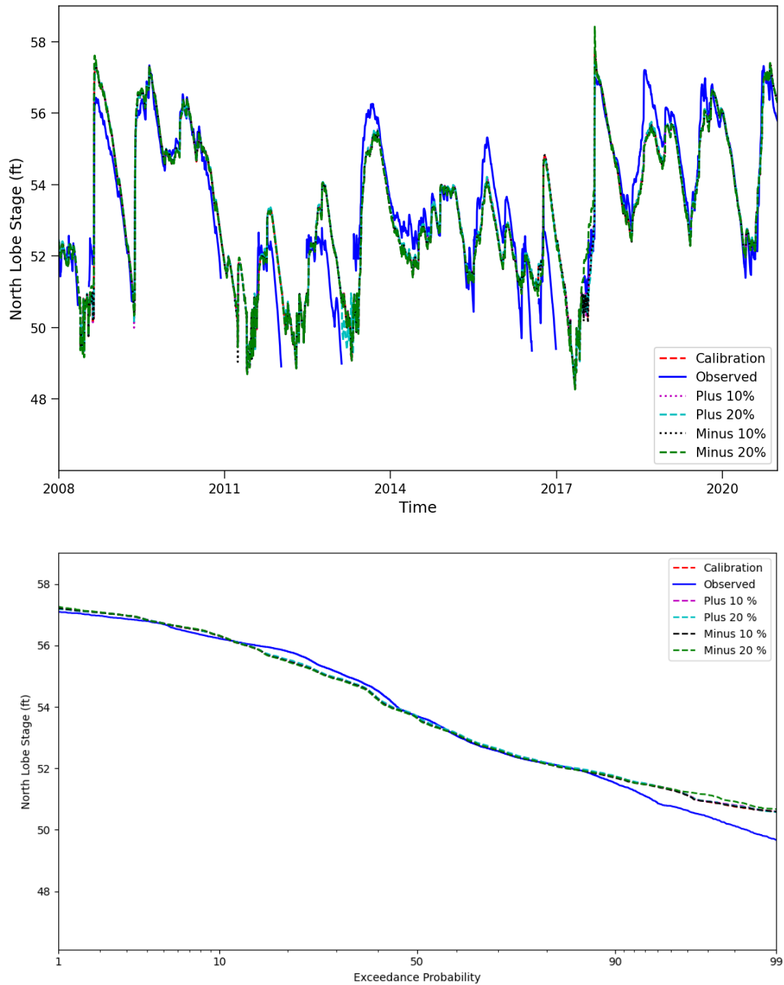
Figure 33. Impact of INFILT on simulated stages of the North Lobe of Prevatt Lake
