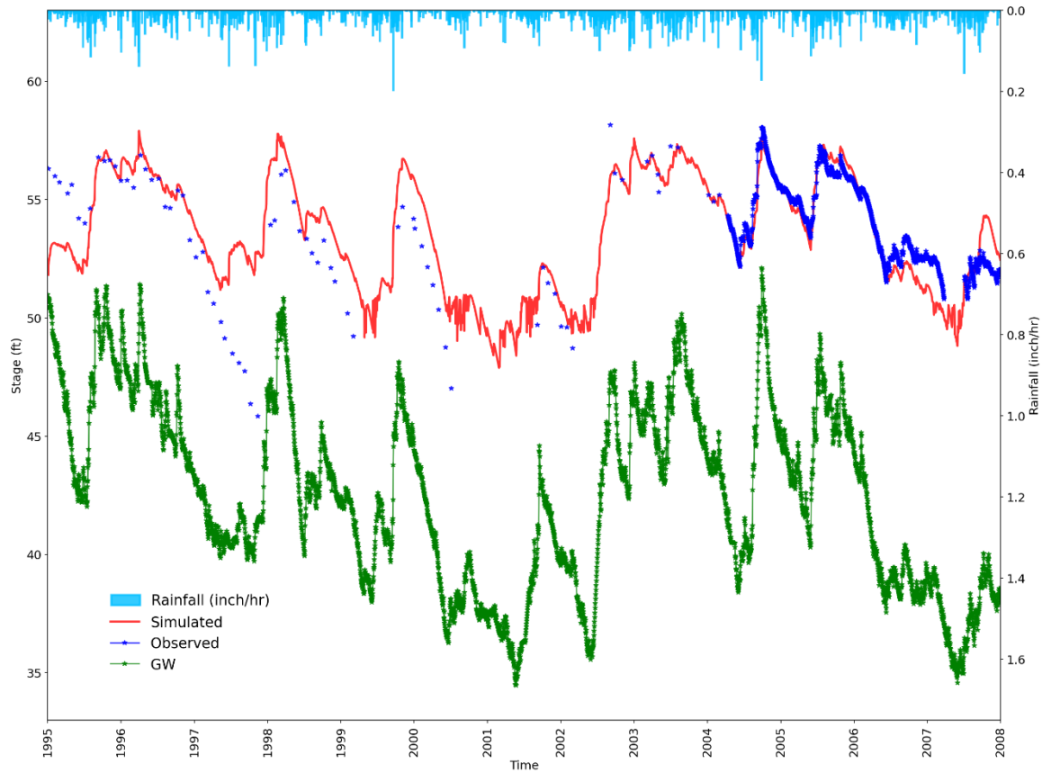
Figure 21. Observed and simulated daily stages for the North Lobe of Prevatt Lake for validation period
