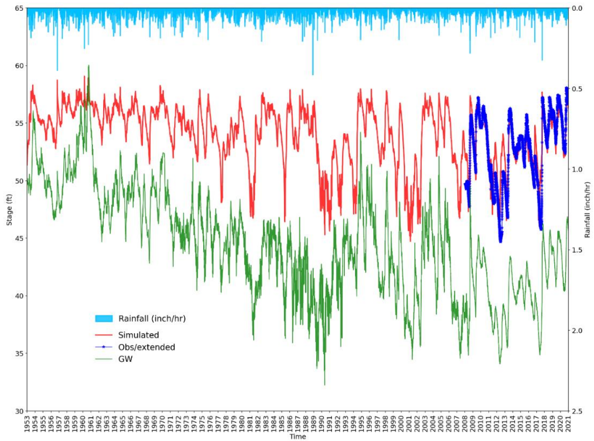
Figure 24. Daily long-term observed and simulated stages of the South Lobe of Prevatt Lake
