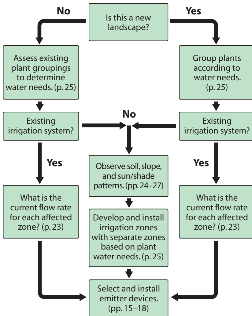
Figure 3.1 Evaluating the Landscape and Irrigation System Flow Chart
