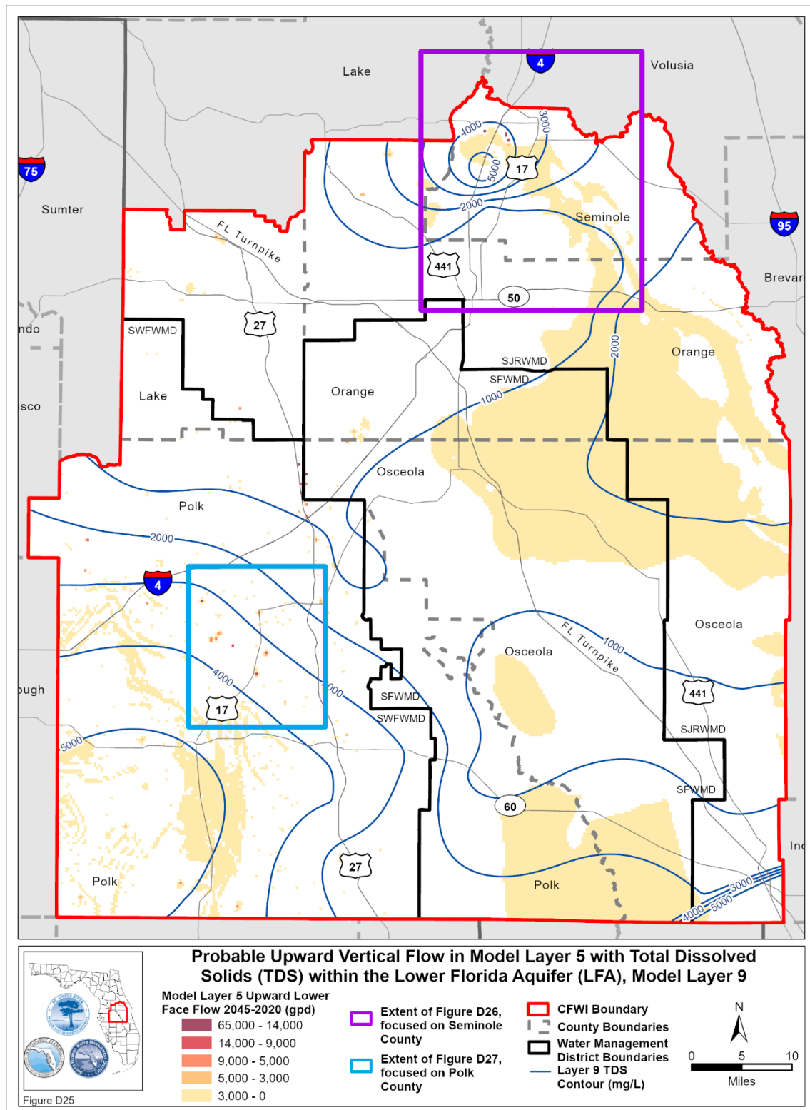
Figure D-25. Potential increased vertical flow through the bottom face of Model Layer 5 between the 2016-2020 Reference Condition and the 2045 Withdrawals Condition with Total Dissolved Solids Concentration Contours in Model Layer 9 (LFA) within the CFWD Planning Area.
