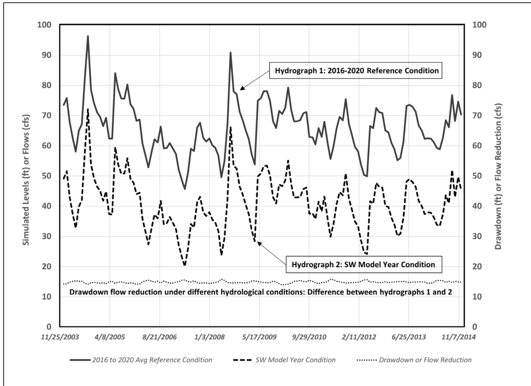
Figure C-7. Illustration showing the estimation of freeboard or deficit for the 2016-2020 Reference Condition using the ECFTXv2.0 model and Surface Water Model.
