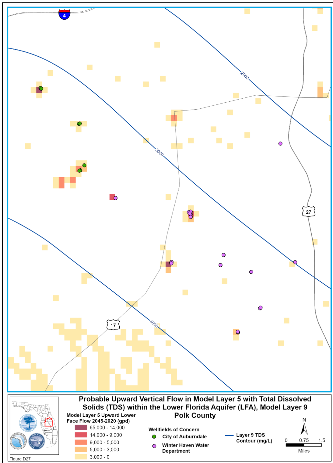
Figure D-27. Potential increased vertical flow through the bottom face of Model Layer 5 between the 2016-2020 Reference Condition and the 2045 Withdrawals Condition with Total Dissolved Solids Concentration Contours in Model Layer 9 (LFA) within Polk County, Florida.
