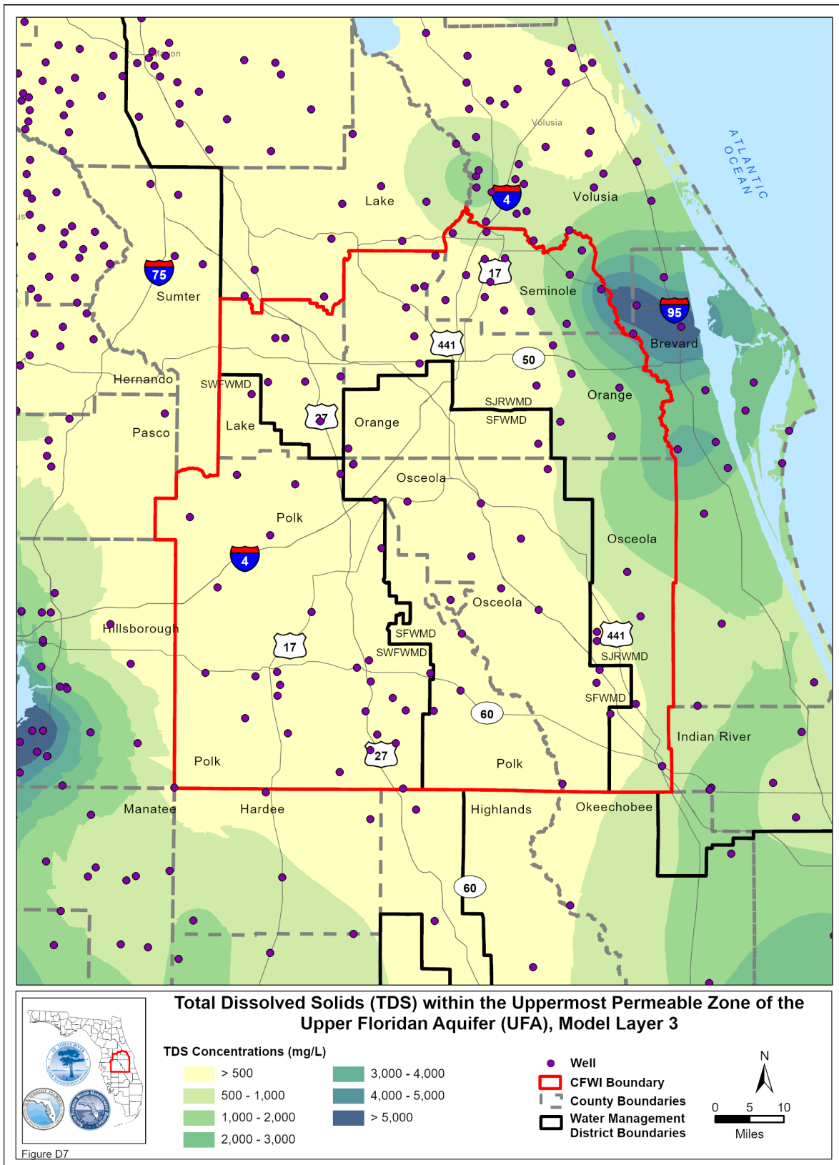
Figure D-7. Total dissolved solids concentrations within the Upper Floridan aquifer (Model Layer 3).
