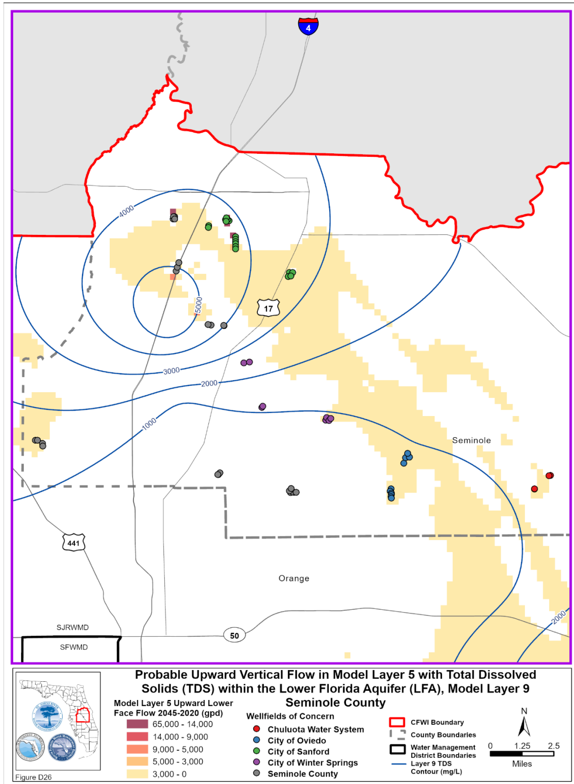
Figure D-26. Potential increased vertical flow through the bottom face of Model Layer 5 between the 2016-2020 Reference Condition and the 2045 Withdrawals Condition with Total Dissolved Solids Concentration Contours in Model Layer 9 (LFA) within Seminole County.
